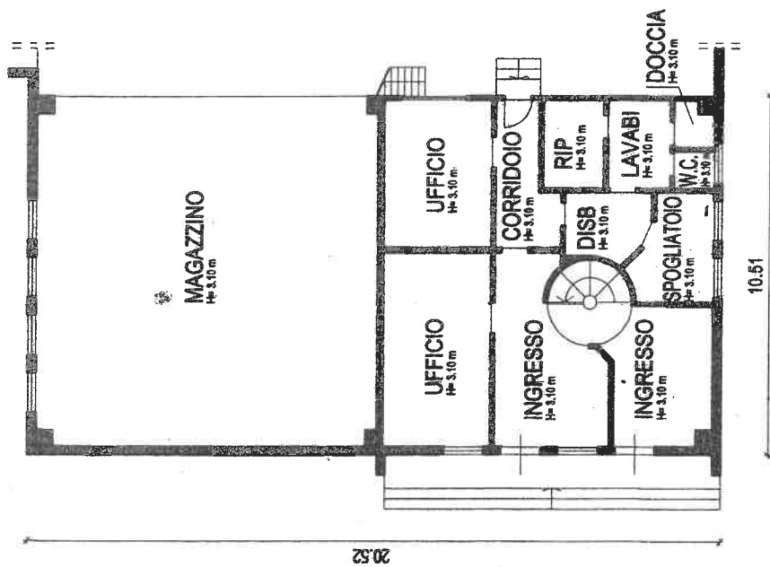
PIANO TERRA H=3.10 - 6.75 m
